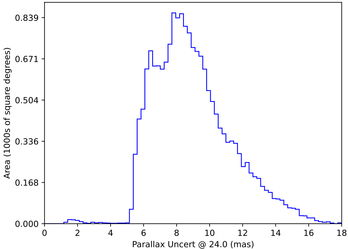
roman_v3.3_10yrs WFD: Parallax Uncert @ 24.0
