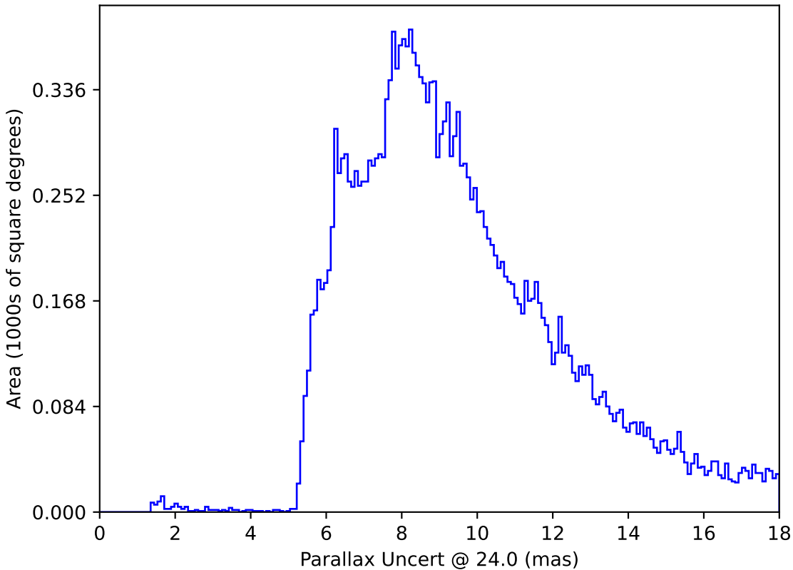
roman_v3.3_10yrs All sky: Parallax Uncert @ 24.0
