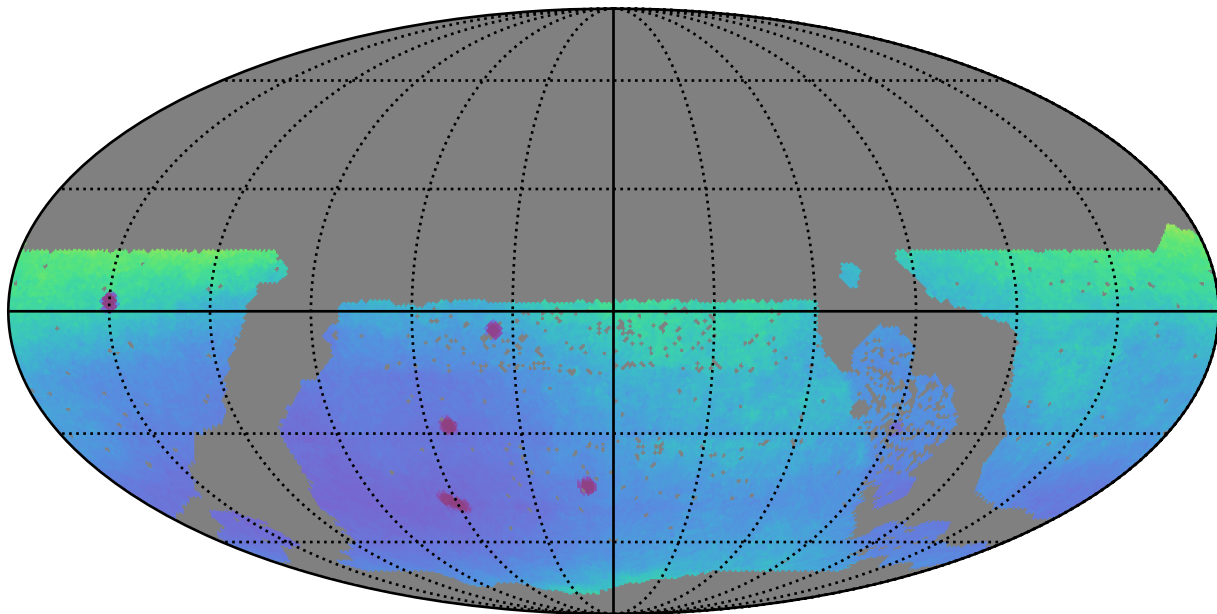
roman_v3.3_10yrs WFD: Parallax Uncert @ 22.4
