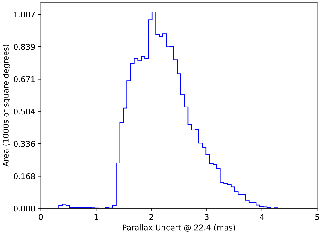
roman_v3.3_10yrs WFD: Parallax Uncert @ 22.4
