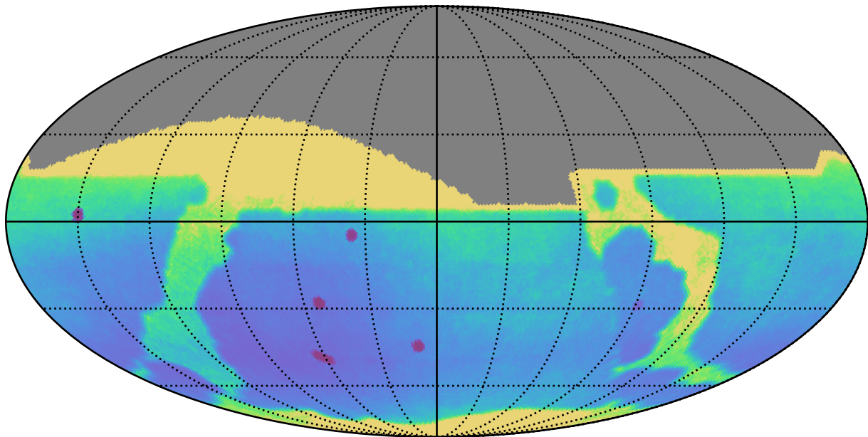
roman_v3.3_10yrs All sky: Parallax Uncert @ 22.4
