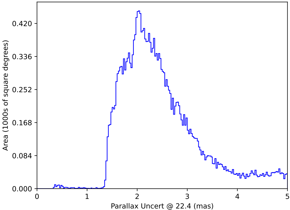
roman_v3.3_10yrs All sky: Parallax Uncert @ 22.4
