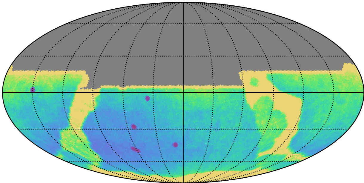
roman_v3.3_10yrs All sky y band only: Parallax Uncert @ 21.3
