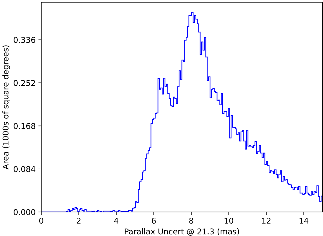
roman_v3.3_10yrs All sky y band only: Parallax Uncert @ 21.3
