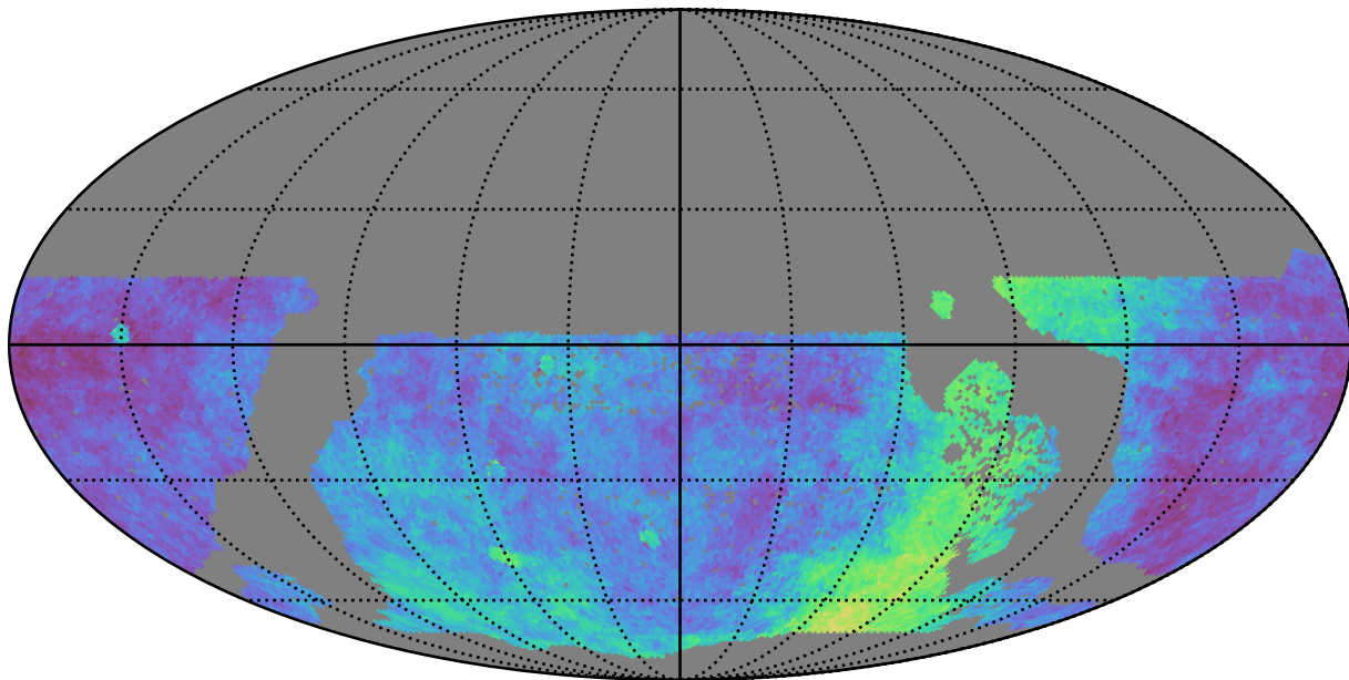
roman_v3.3_10yrs WFD: Parallax Coverage @ 24.0
