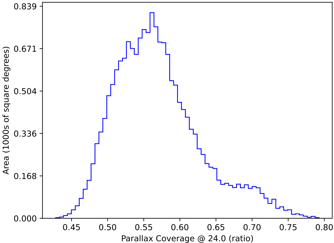
roman_v3.3_10yrs WFD: Parallax Coverage @ 24.0
