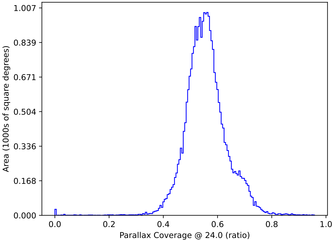
roman_v3.3_10yrs All sky: Parallax Coverage @ 24.0
