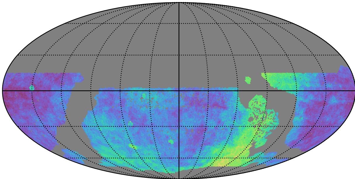
roman_v3.3_10yrs WFD: Parallax Coverage @ 22.4
