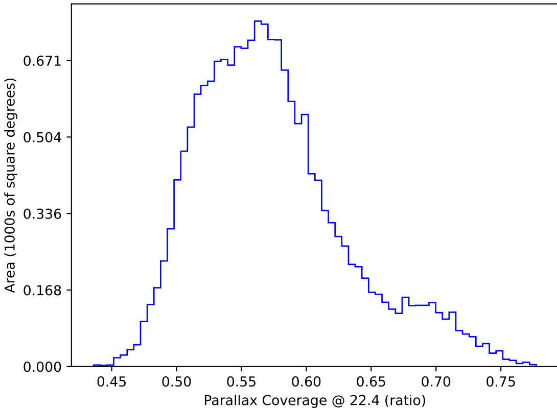
roman_v3.3_10yrs WFD: Parallax Coverage @ 22.4
