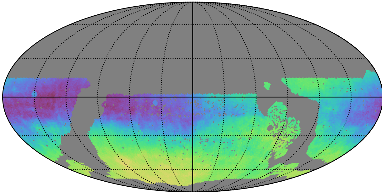
roman_v3.3_10yrs WFD: Parallax-DCR degeneracy @ 24.0
