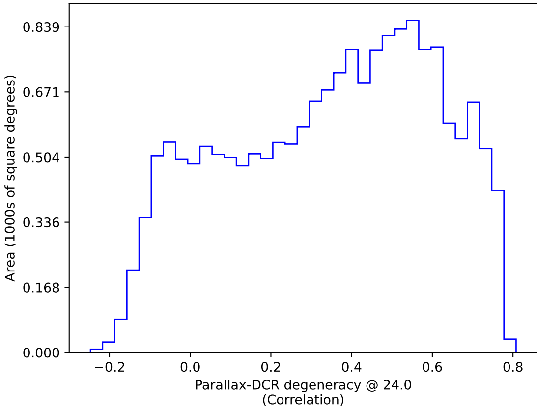
roman_v3.3_10yrs WFD: Parallax-DCR degeneracy @ 24.0
