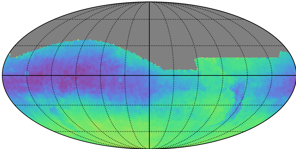
roman_v3.3_10yrs All sky: Parallax-DCR degeneracy @ 24.0
