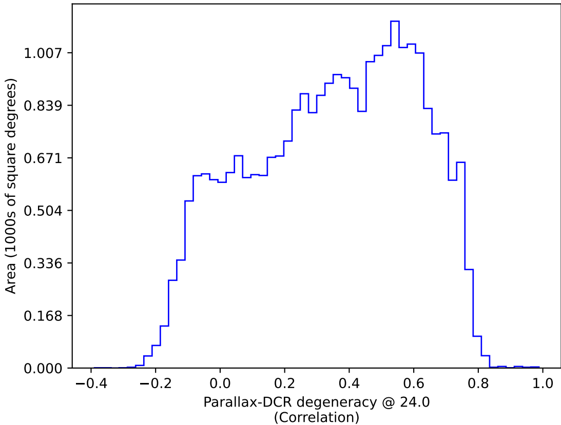
roman_v3.3_10yrs All sky: Parallax-DCR degeneracy @ 24.0
