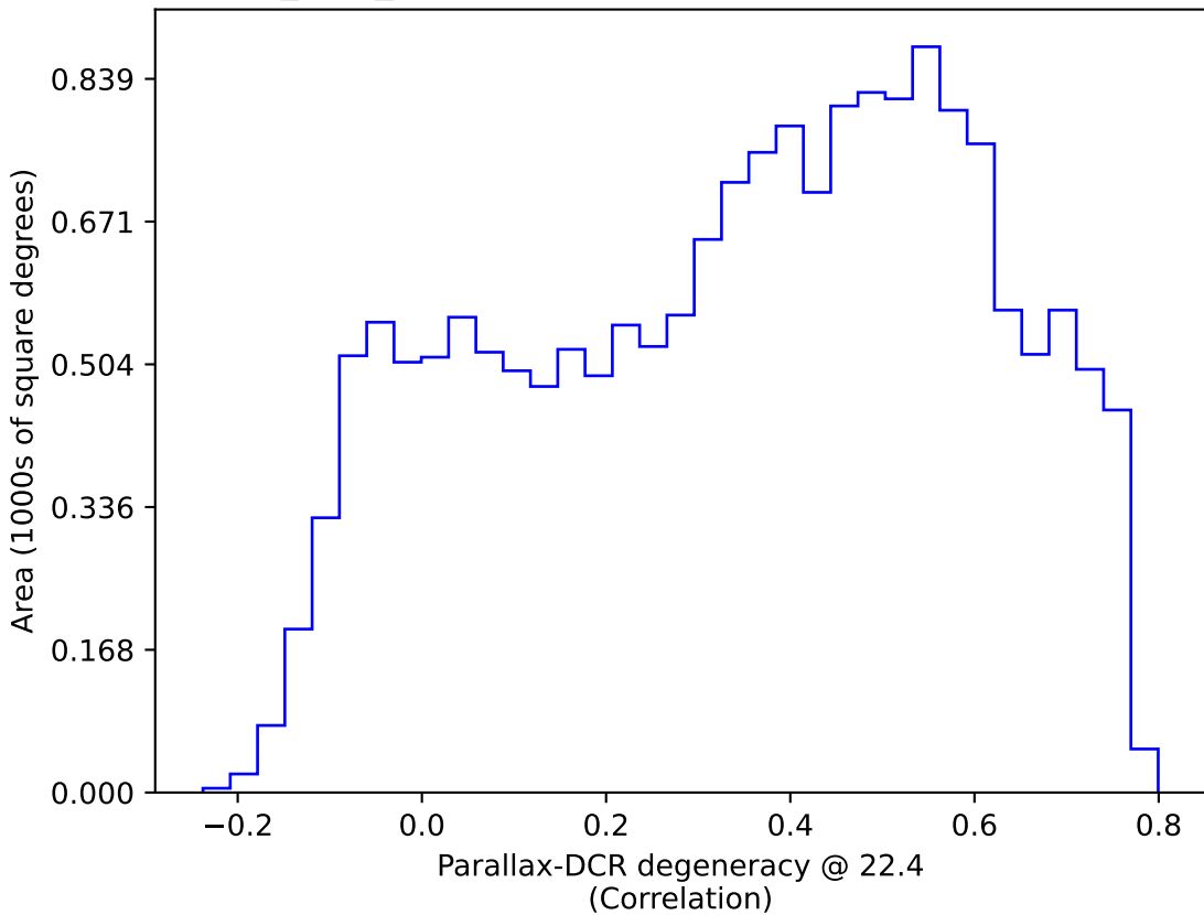
roman_v3.3_10yrs WFD: Parallax-DCR degeneracy @ 22.4
