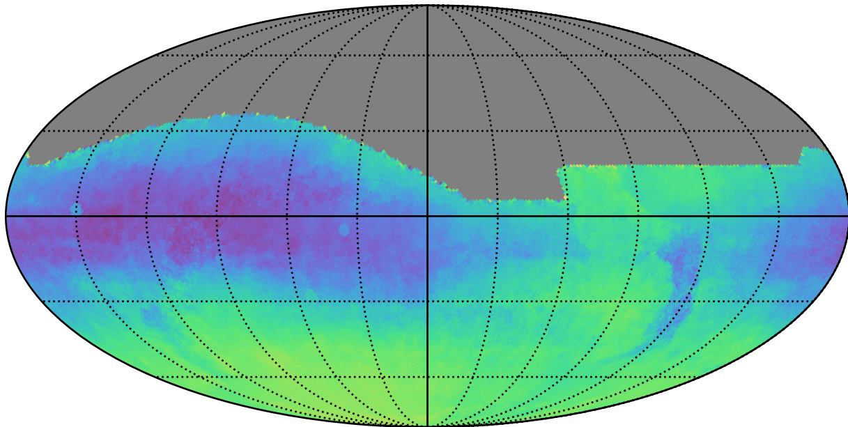
roman_v3.3_10yrs All sky: Parallax-DCR degeneracy @ 22.4
