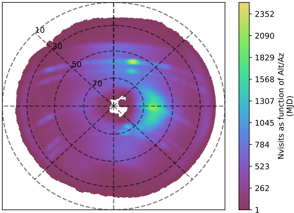
roman_v3.3_10yrs z band: Nvisits as function of Alt/Az
