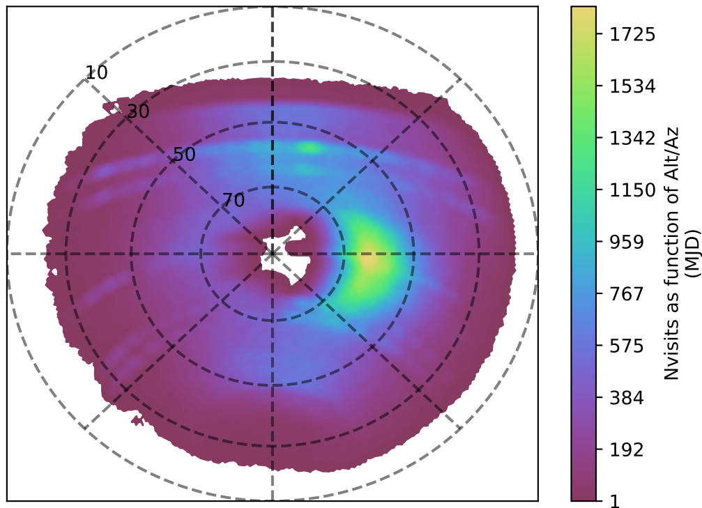
roman_v3.3_10yrs y band: Nvisits as function of Alt/Az
