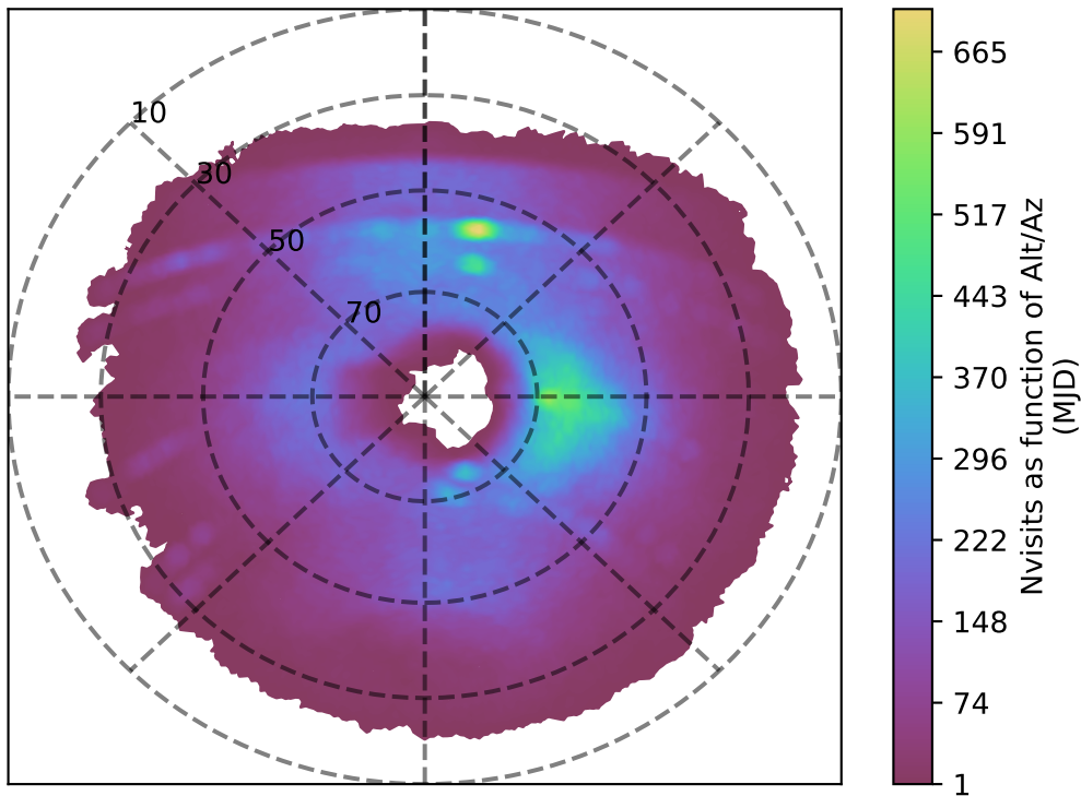
roman_v3.3_10yrs u band: Nvisits as function of Alt/Az
