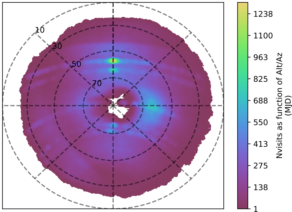
roman_v3.3_10yrs g band: Nvisits as function of Alt/Az
