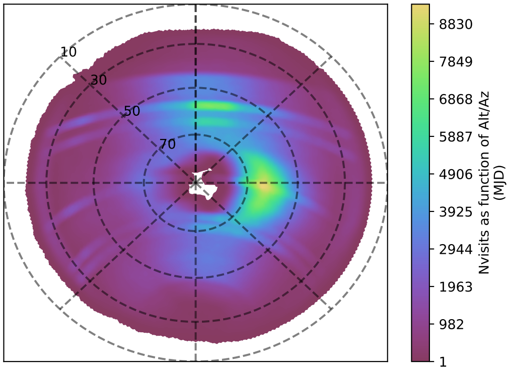
roman_v3.3_10yrs all bands: Nvisits as function of Alt/Az
