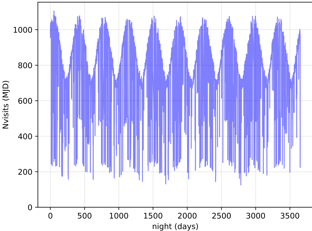
roman_v3.3_10yrs All visits: Nvisits
