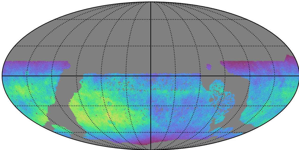
roman_v3.3_10yrs WFD z band: Normalized Teff
