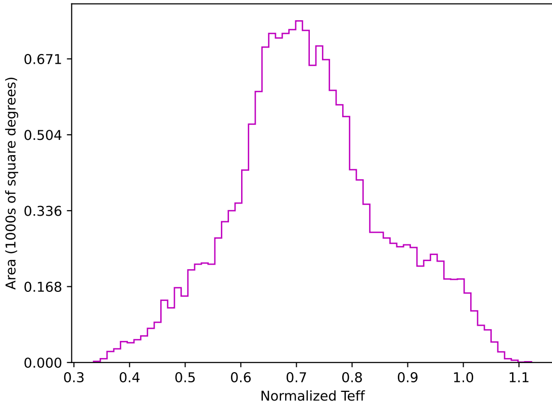
roman_v3.3_10yrs WFD z band: Normalized Teff
