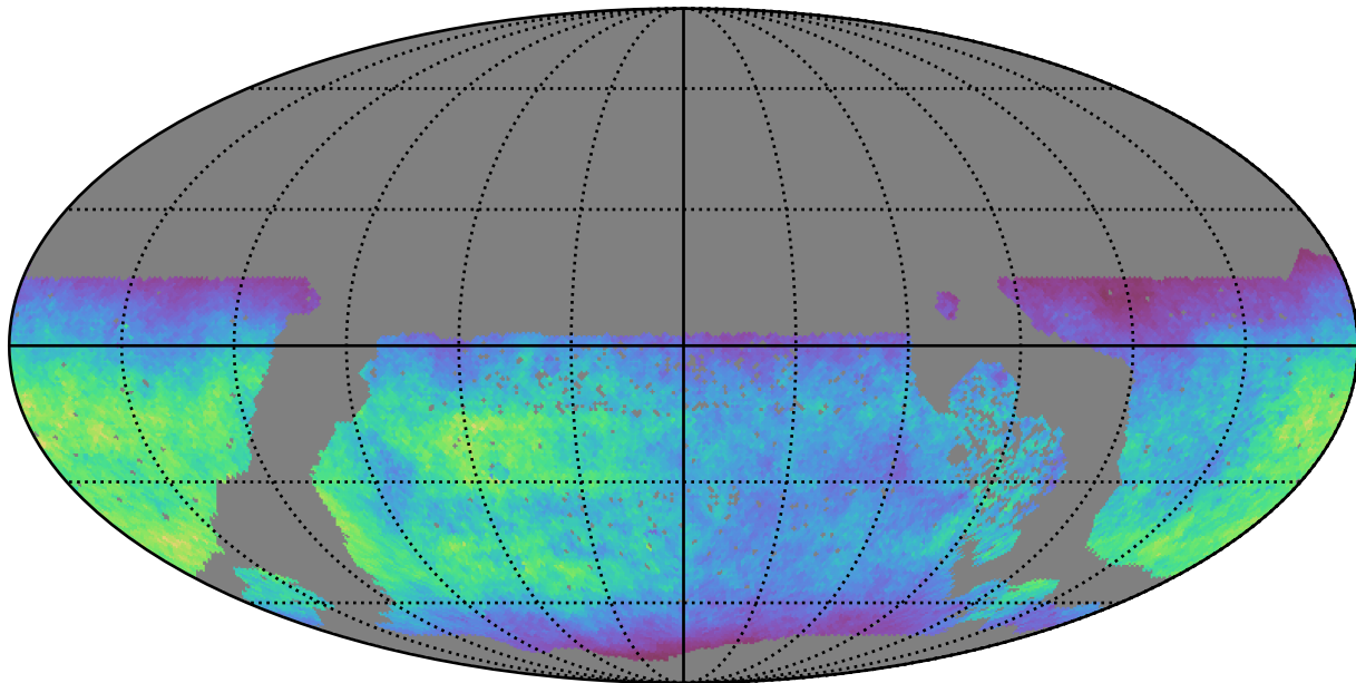
roman_v3.3_10yrs WFD u band: Normalized Teff
