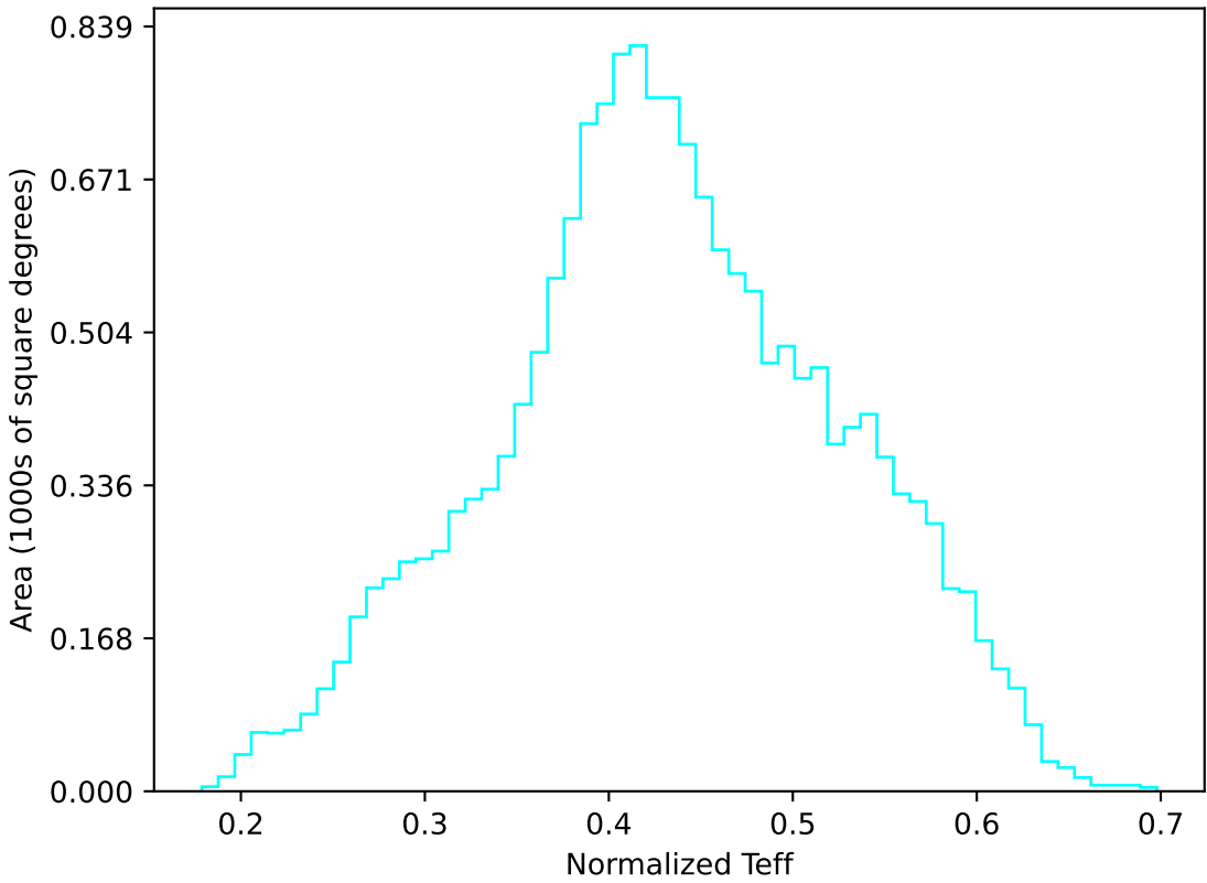
roman_v3.3_10yrs WFD u band: Normalized Teff
