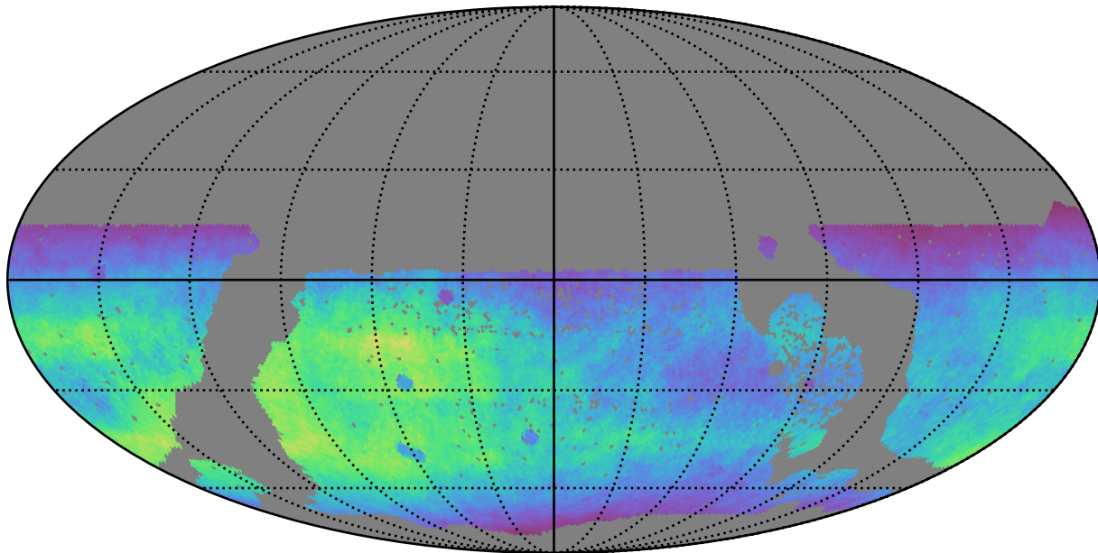
roman_v3.3_10yrs WFD r band: Normalized Teff
