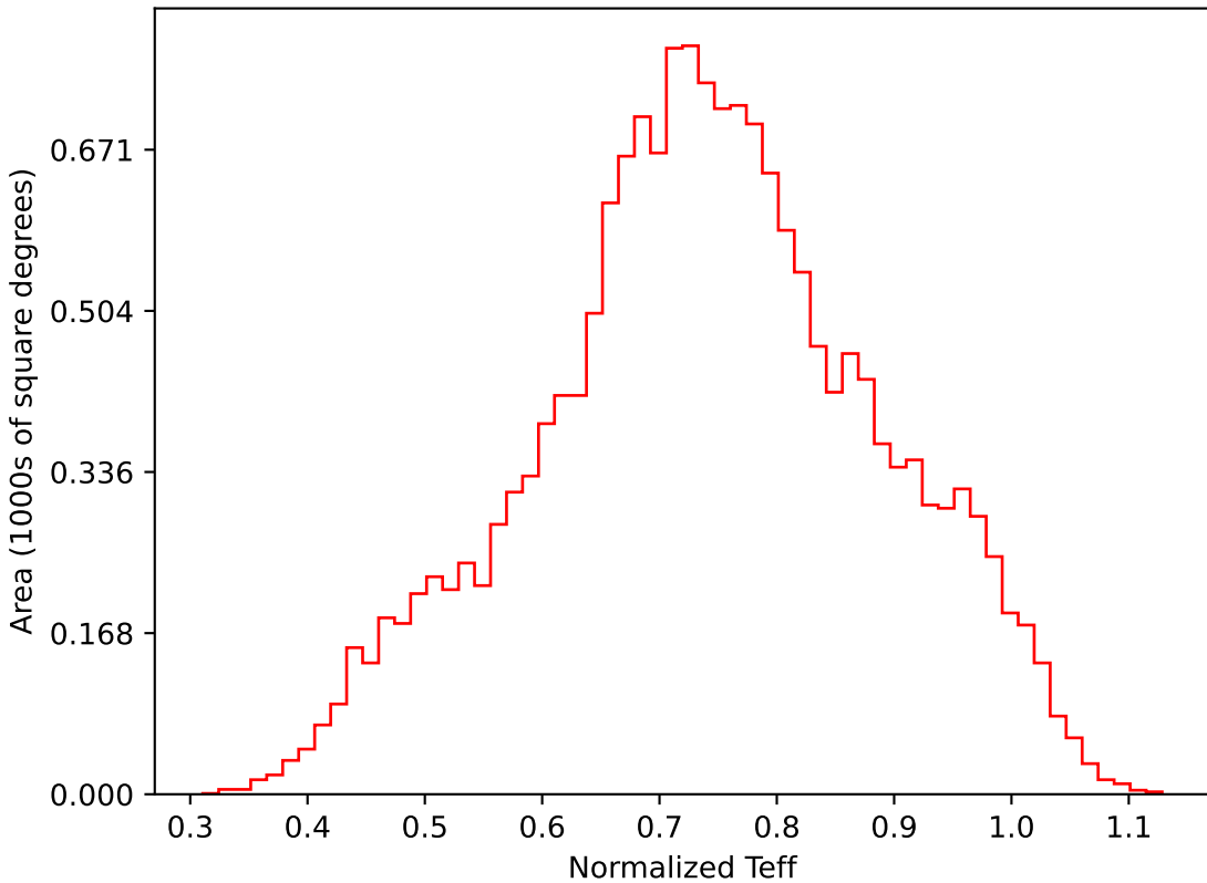
roman_v3.3_10yrs WFD i band: Normalized Teff
