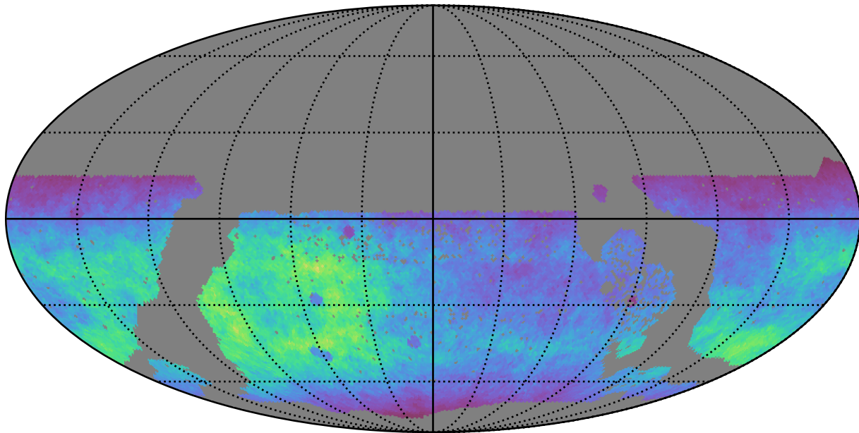
roman_v3.3_10yrs WFD g band: Normalized Teff
