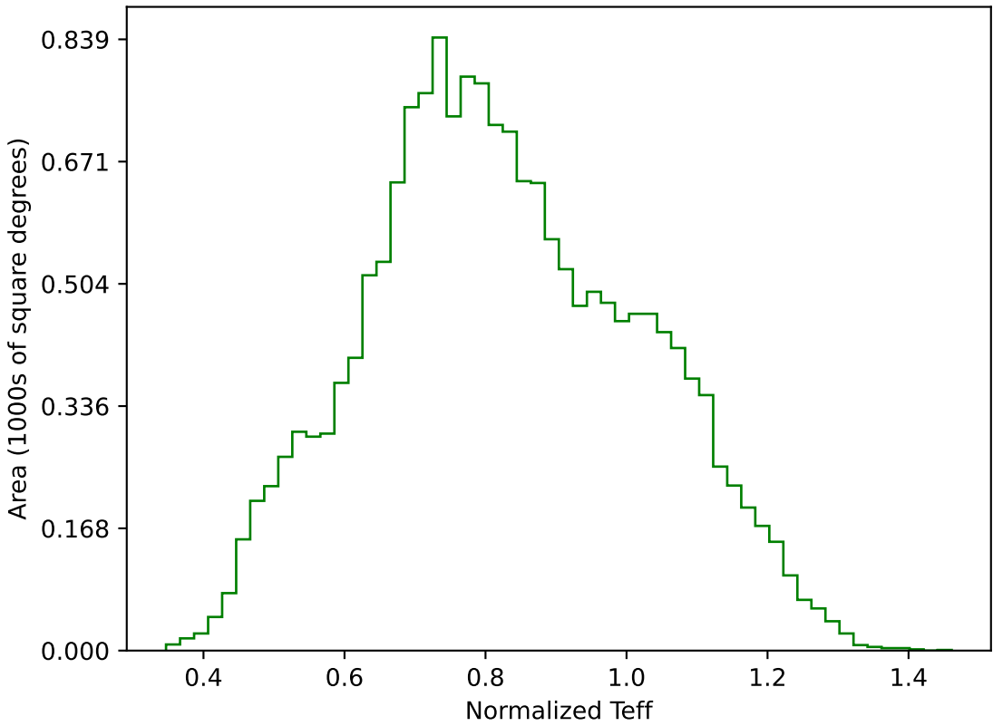
roman_v3.3_10yrs WFD g band: Normalized Teff
