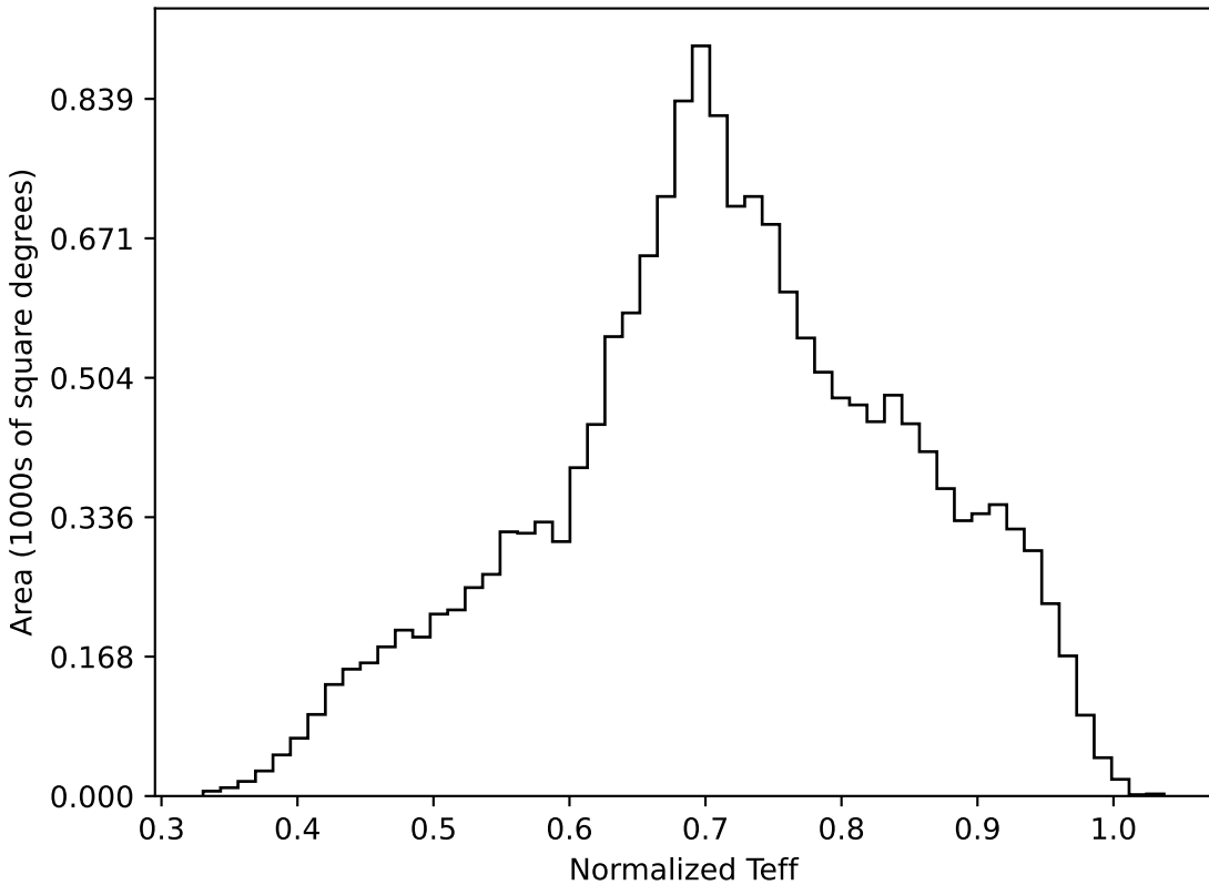
roman_v3.3_10yrs WFD all bands: Normalized Teff
