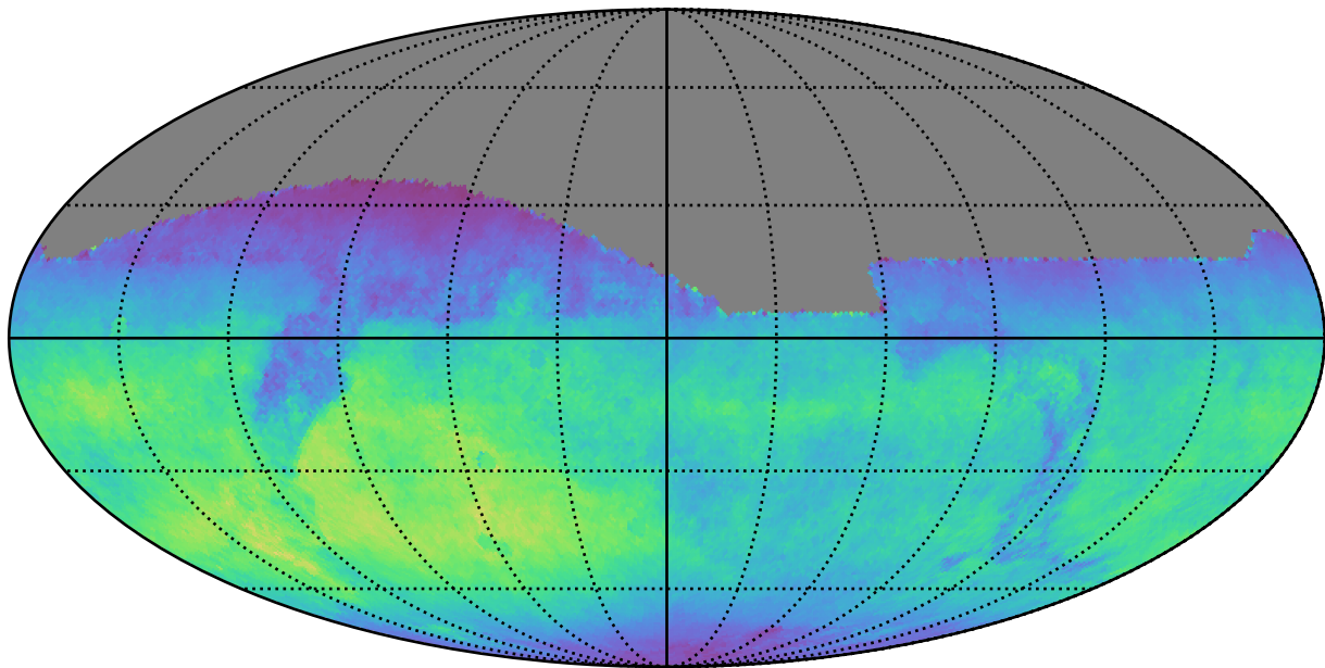
roman_v3.3_10yrs All sky z band: Normalized Teff
