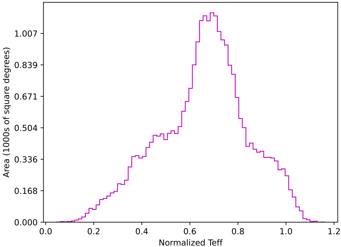
roman_v3.3_10yrs All sky z band: Normalized Teff
