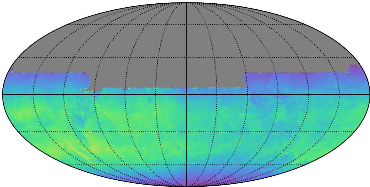
roman_v3.3_10yrs All sky y band: Normalized Teff
