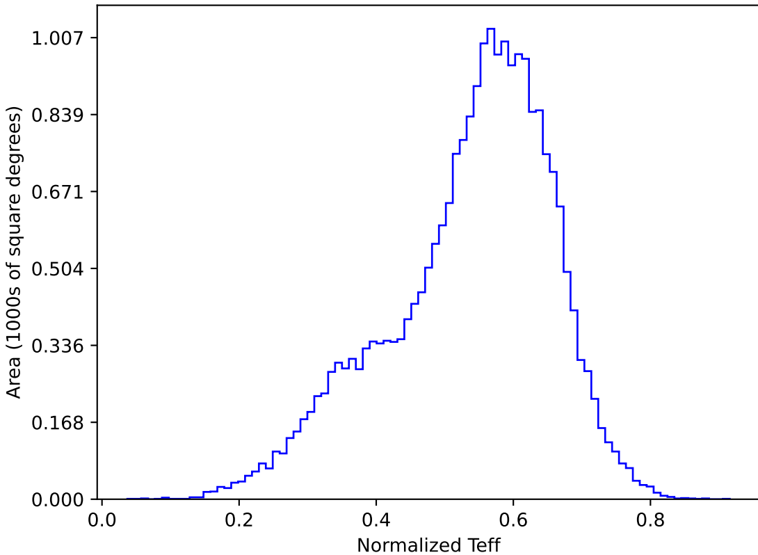
roman_v3.3_10yrs All sky y band: Normalized Teff
