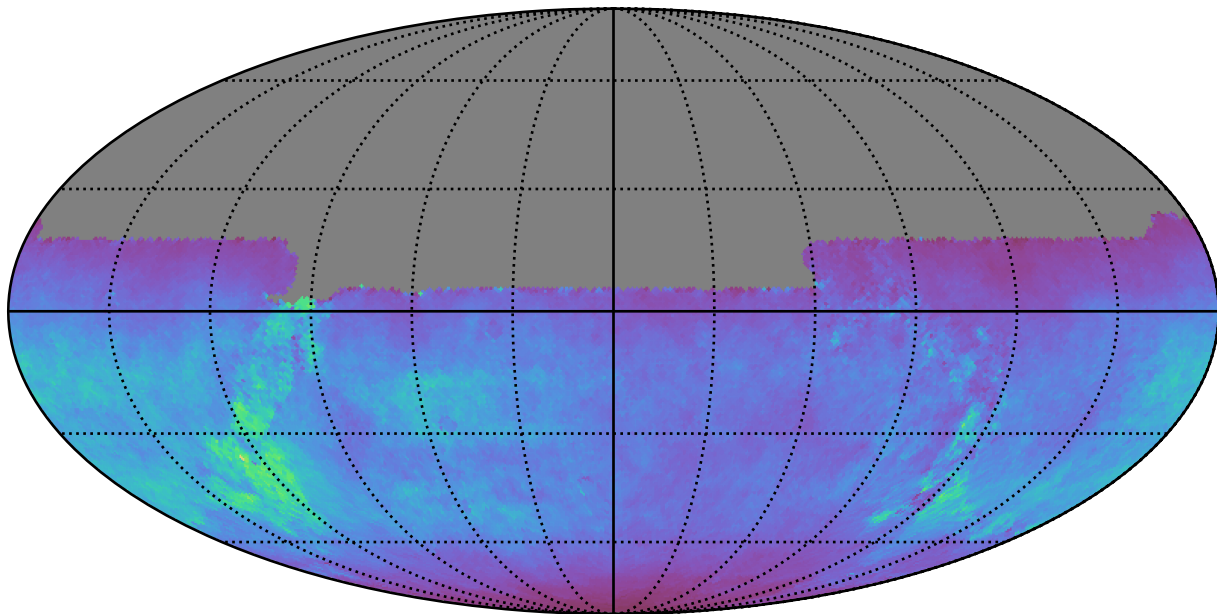
roman_v3.3_10yrs All sky u band: Normalized Teff
