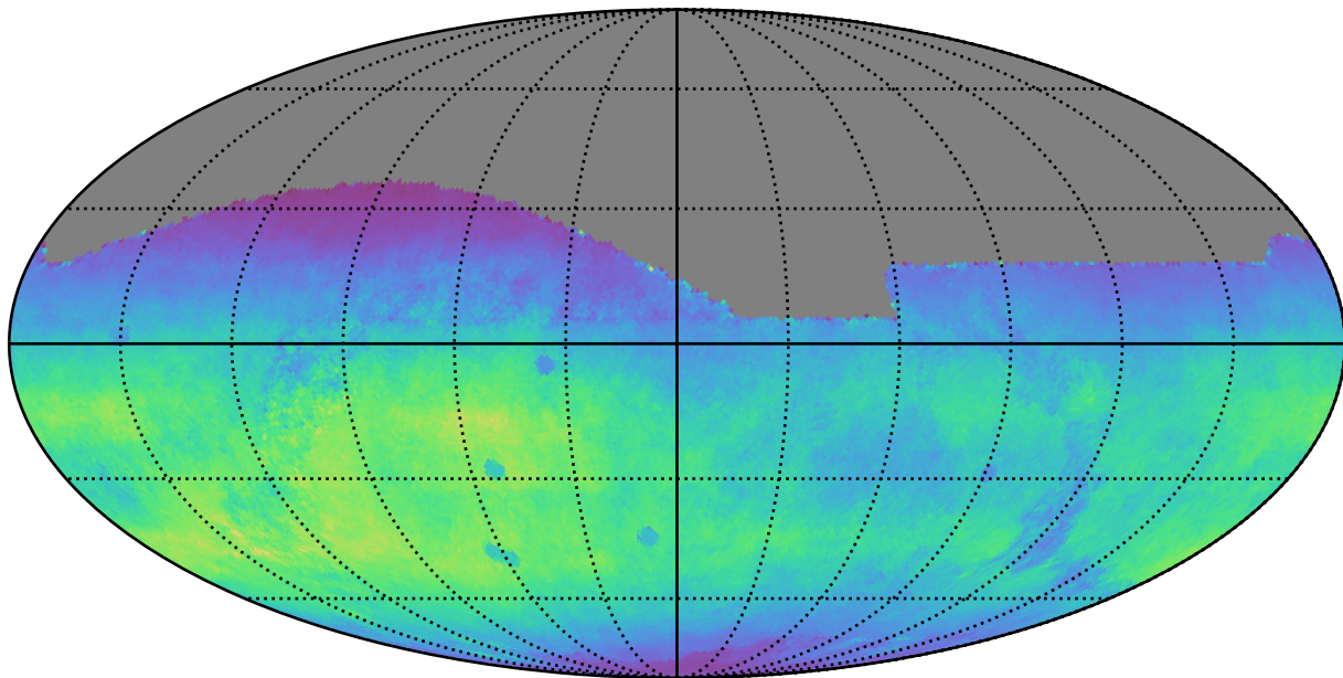
roman_v3.3_10yrs All sky r band: Normalized Teff
