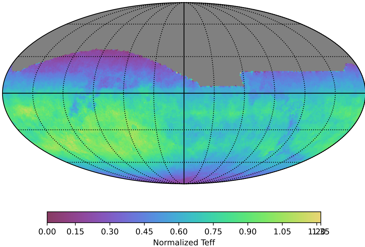
roman_v3.3_10yrs All sky i band: Normalized Teff
