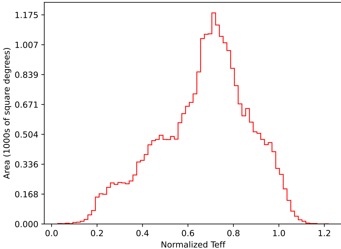
roman_v3.3_10yrs All sky i band: Normalized Teff
