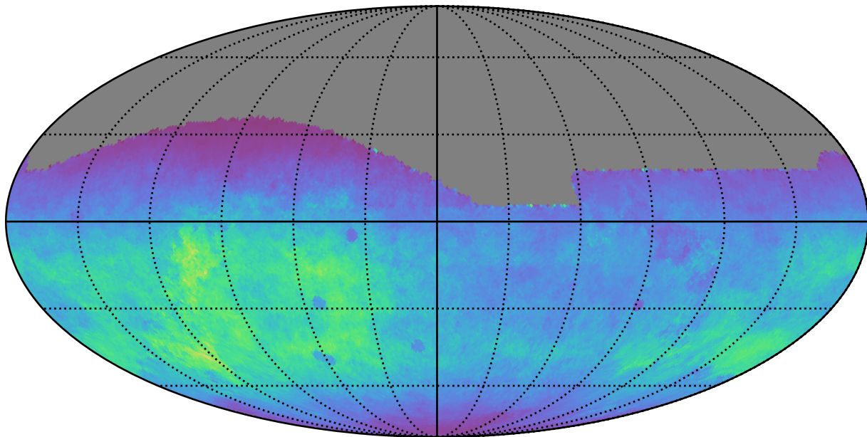
roman_v3.3_10yrs All sky g band: Normalized Teff
