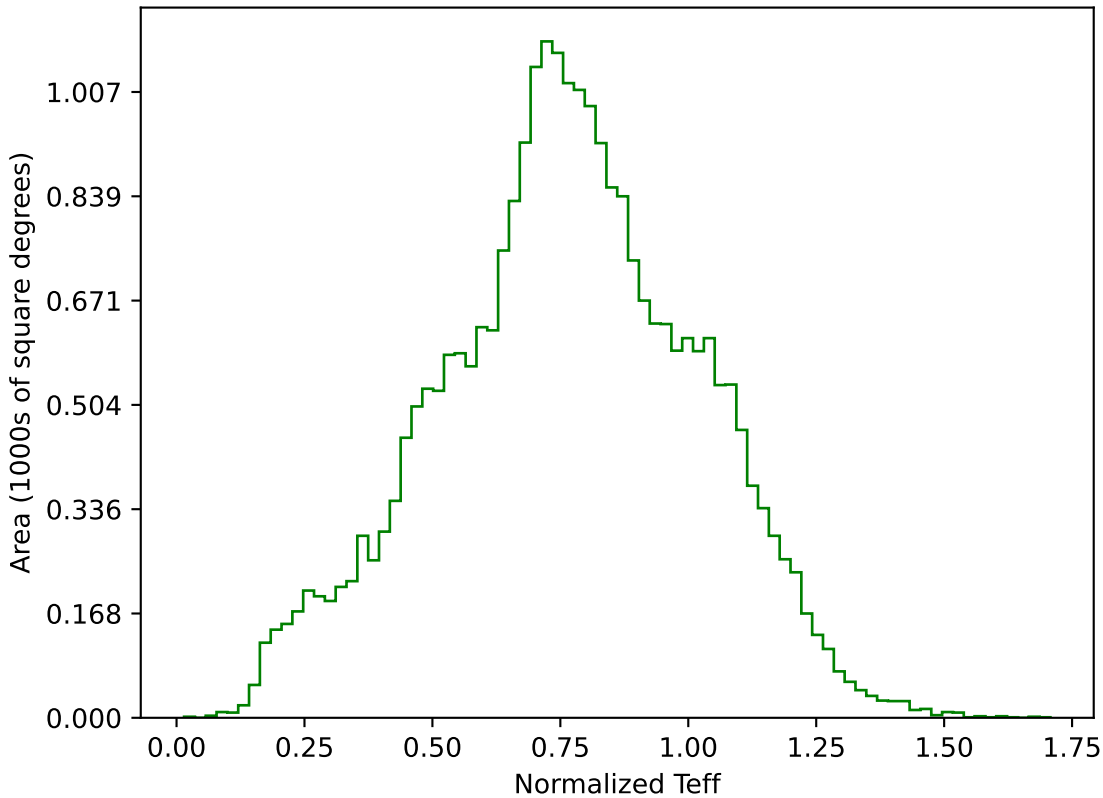
roman_v3.3_10yrs All sky g band: Normalized Teff
