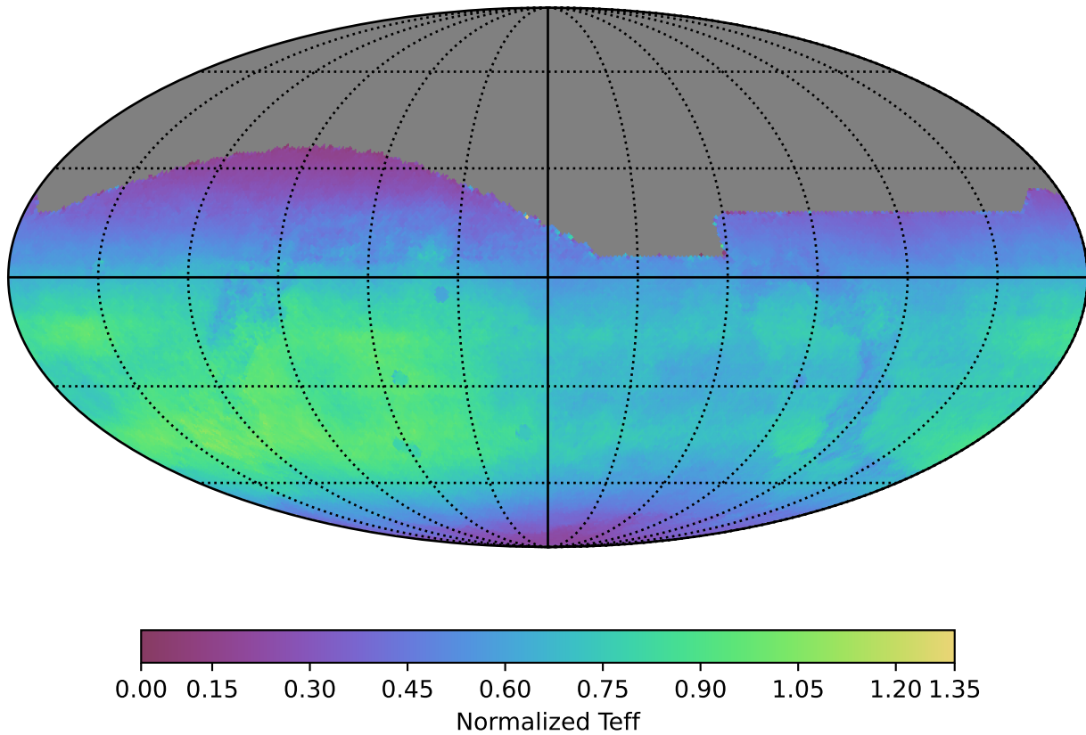
roman_v3.3_10yrs All sky all bands: Normalized Teff
