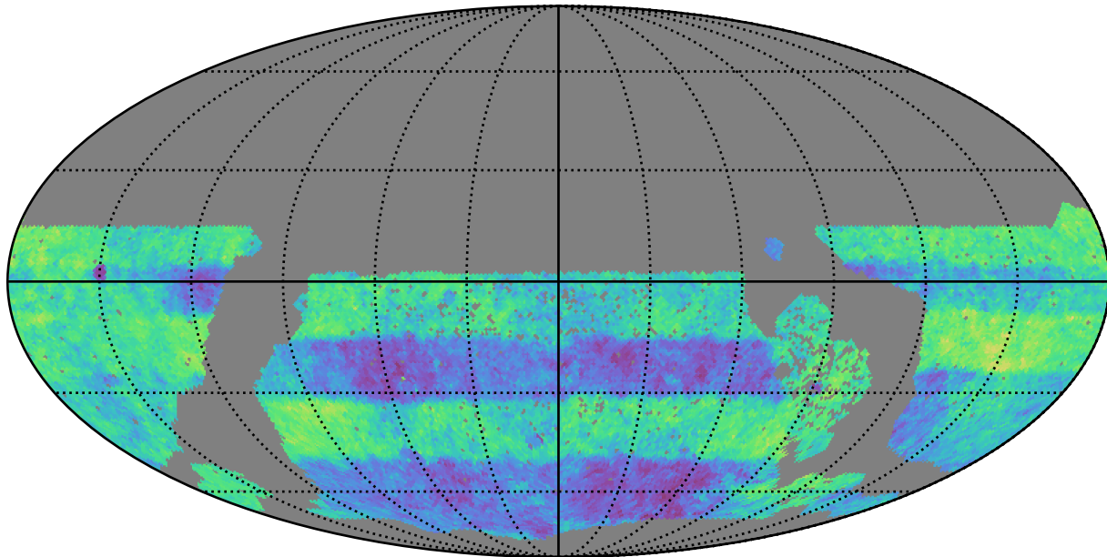
roman_v3.3_10yrs WFD: Normalized Proper Motion Uncert @ 24.0
