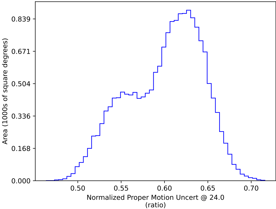
roman_v3.3_10yrs WFD: Normalized Proper Motion Uncert @ 24.0
