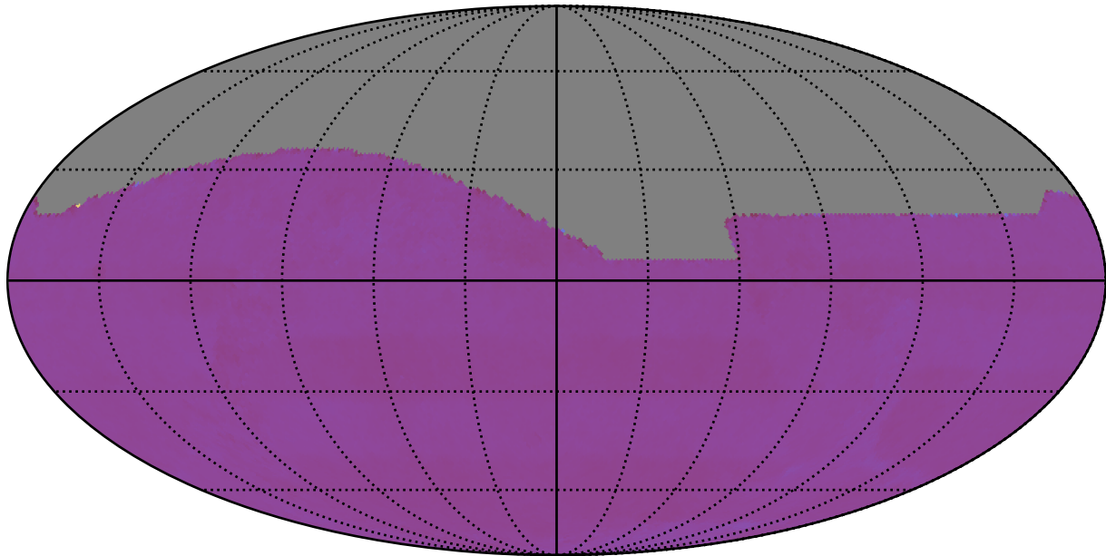
roman_v3.3_10yrs All sky: Normalized Proper Motion Uncert @ 24.0
