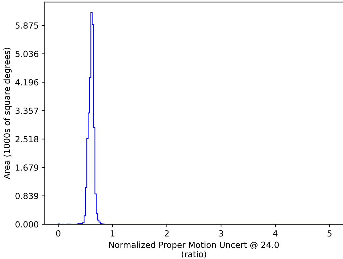
roman_v3.3_10yrs All sky: Normalized Proper Motion Uncert @ 24.0
