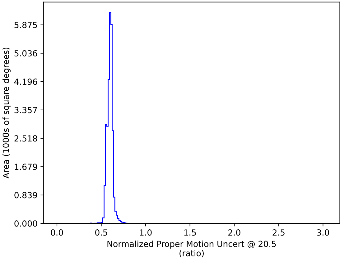
roman_v3.3_10yrs All sky: Normalized Proper Motion Uncert @ 20.5
